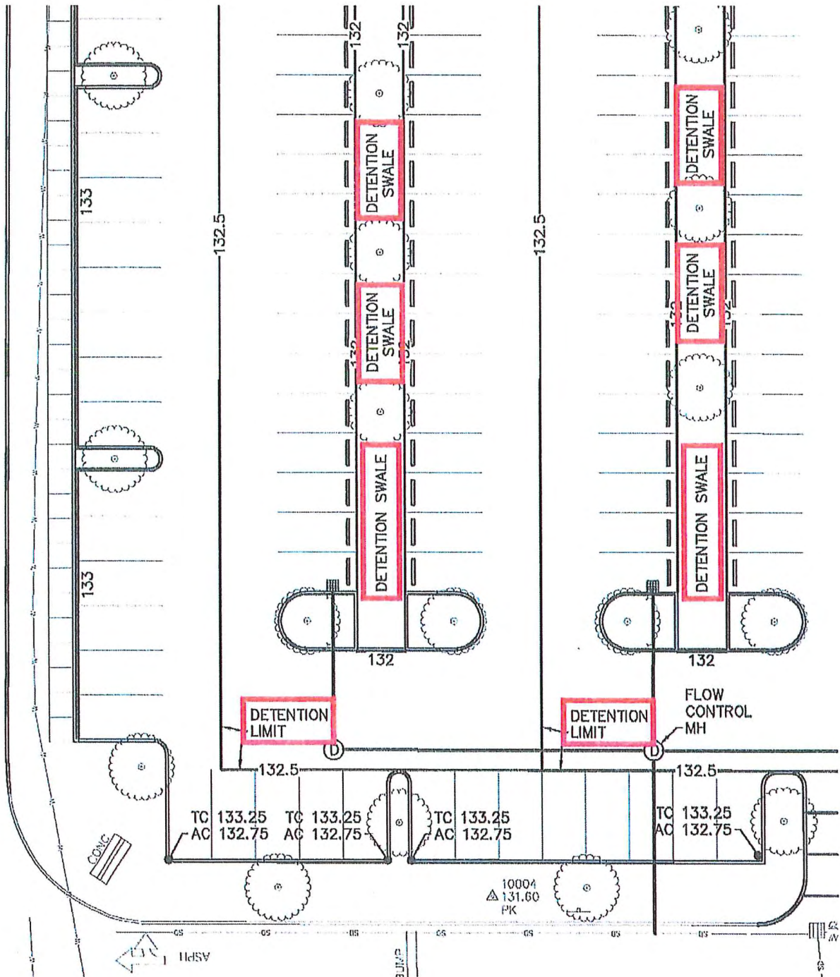
Figure 5-9 | Parking Lot Swale Detention
